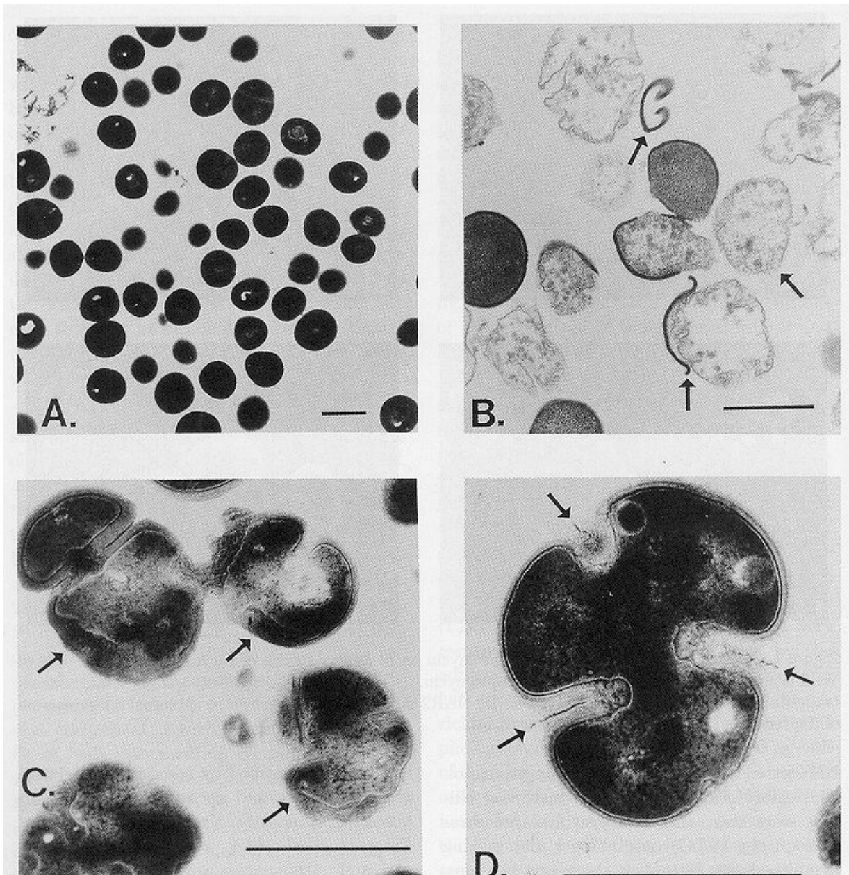
Figure 2. TEM demonstrating effects of daptomycin on S. aureus strains of varying susceptibilities. (A) Wild-type (susceptible) control with no daptomycin. (B) Wild-type exposed to lethal concentration of daptomycin (500 \mu\text{g}/\text{mL} , 3 h). Note partial and total loss of cell wall and developing ghost cells. (C) and (D) DAR2 strain (resistant) grown in sublethal concentration of daptomycin (50 \mu\text{g}/\text{mL} , 24 h). Note loss of symmetry and extrusion of amorphous material. Bar = 1 \mu\text{m} .
